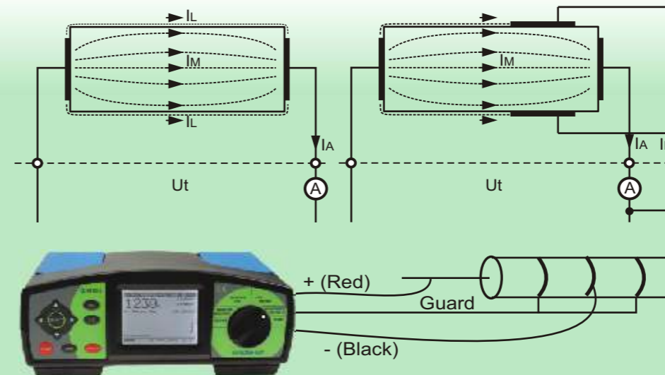
Connection of GUARD terminal to measured object (an example for measuring cable insulation is shown)
